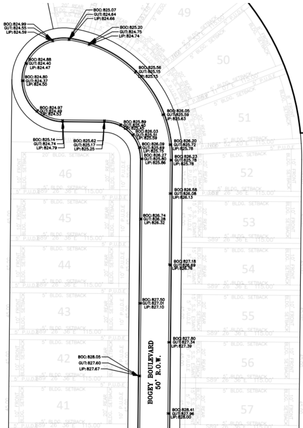
Example of Roadway Grading shown above
