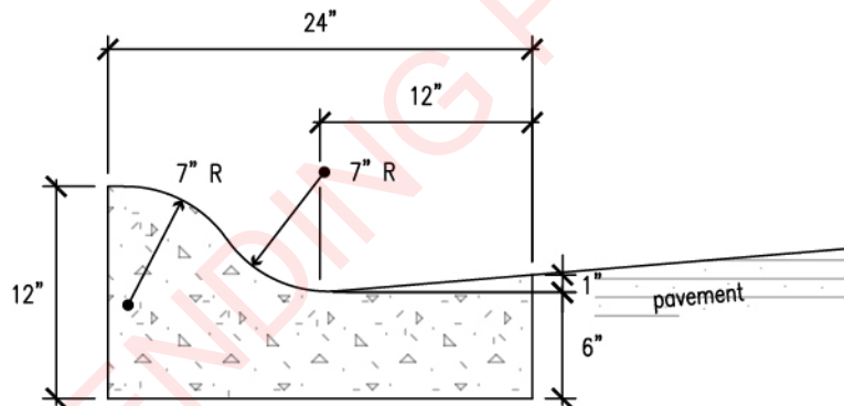
24" Rolled Curb
