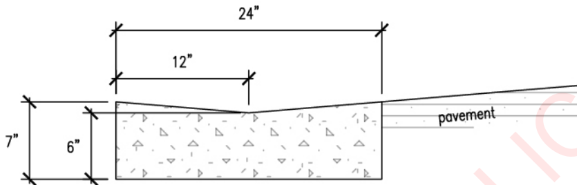
24" Valley Curb
